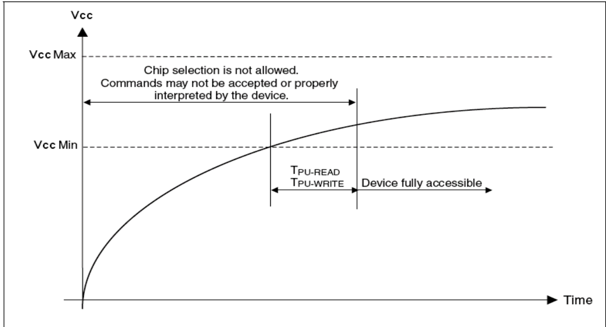
Power-up Timing
