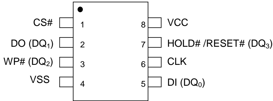
8 - LEAD SOP
